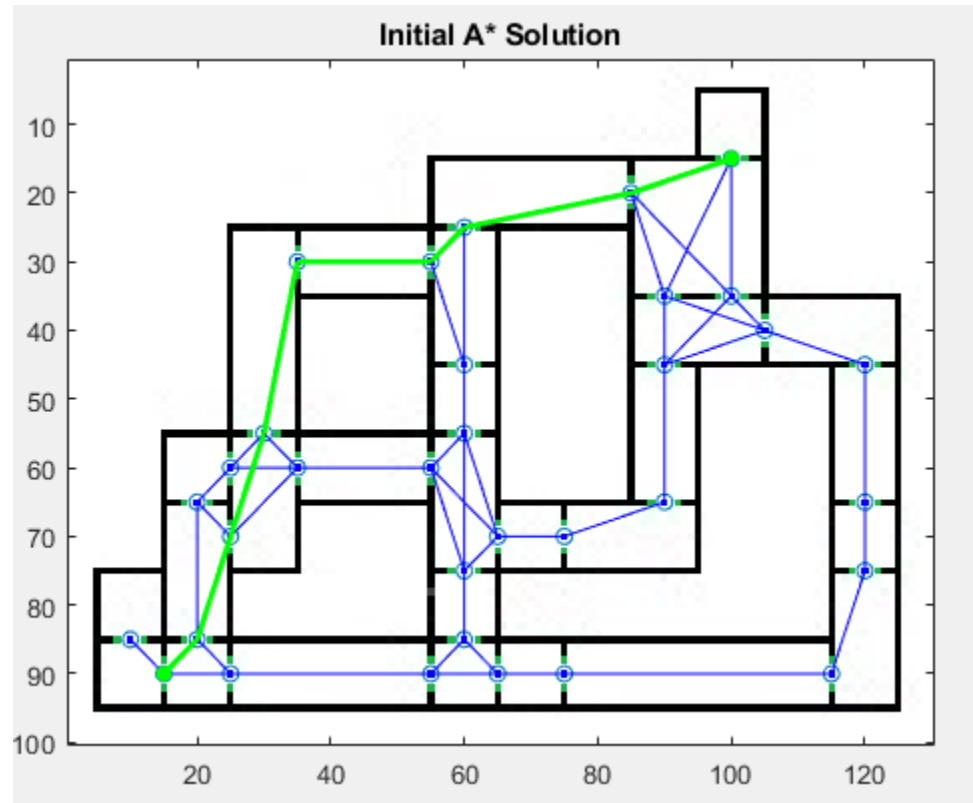
The initial A* solution starting in the bottom left corner traveling to the top right
